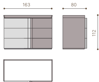
CASSETTIERA CHEST OF DRAWERS
